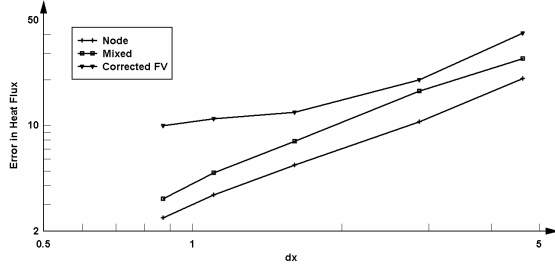
Figure 20. Accuracy of Discrete Calculus and finite volume methods.
