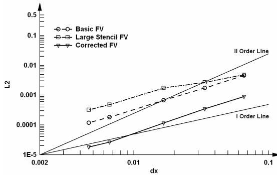
Figure 6. Spatial accuracy of classical FV methods.
