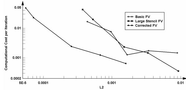
Figure 17. Cost incurred by FV methods
