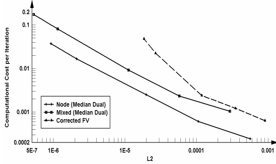
Figure 16. Computational cost incurred for a desired accuracy level
