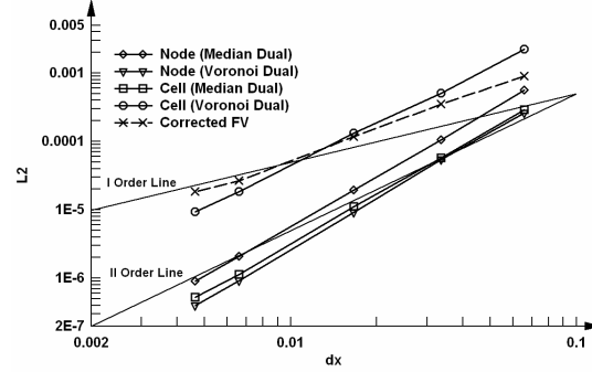
Figure 11. Spatial accuracy of Discrete Calculus methods
