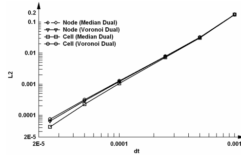
Figure 14. Temporal accuracy of DC methods.
