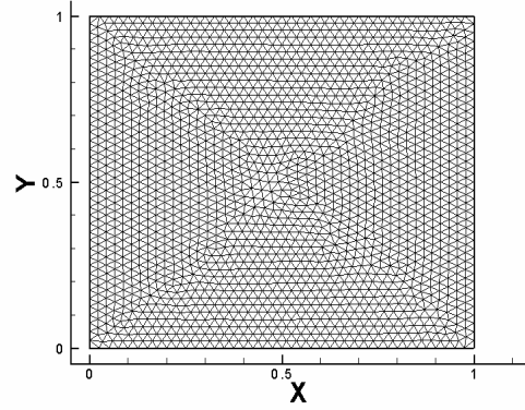
Figure 5. Typical mesh used for convergence studies.
