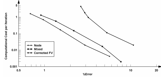
Figure 21. Cost for a desired accuracy for the Crank shaft test case.
