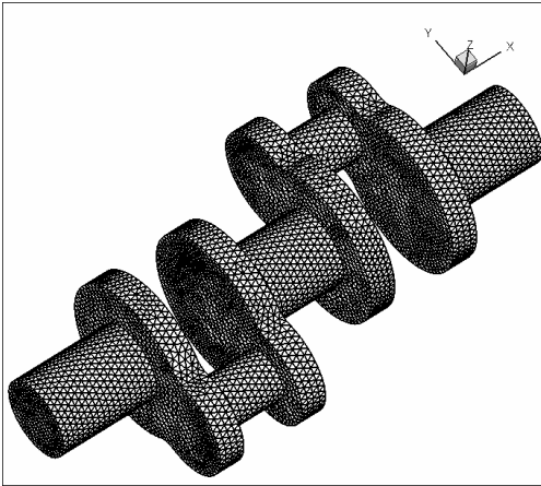
Figure 18. Crank Shaft Mesh
