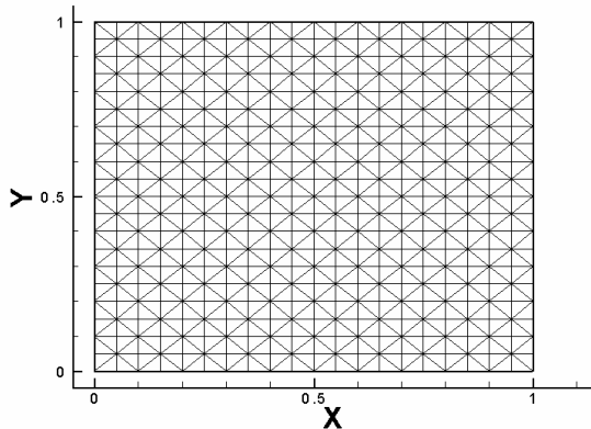
Figure 8. Mesh with different diffusivities on either side of the interface ( x=0.5 ).
