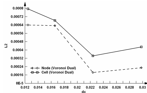
Figure 13. Accuracy of Voronoi Dual Methods on stretched meshes
