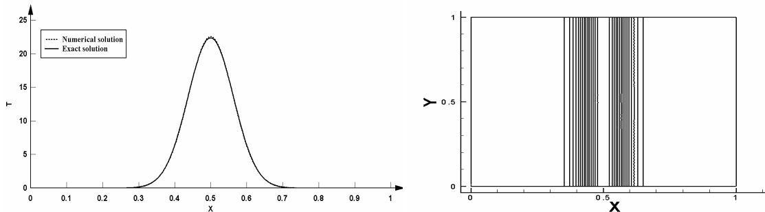
Figure 15. Solution to the unsteady diffusion problem at t=0.002 .
