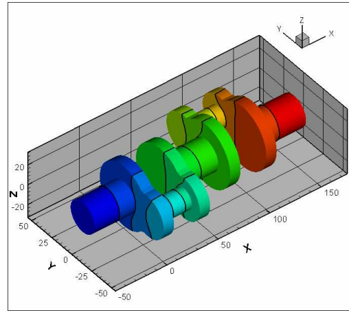
Figure 19. Temperature contours along the crankshaft.
