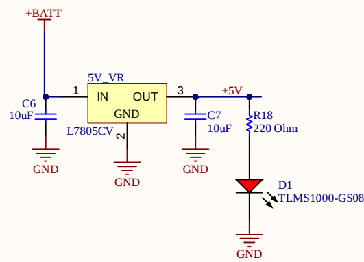
5V Voltage Regulator
