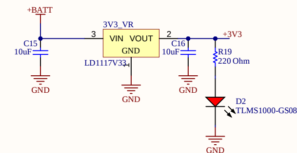
3V3 Voltage Regulator
