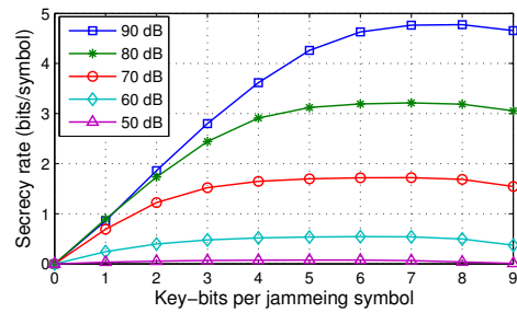
Fig. 8. Secrecy rate versus the number of key bits per jamming symbol ( k ) for various values of the total SNR, when P + P_J = 1 , both Bob and Eve have 10 bit A/Ds, and the quality of both channels is the same.
