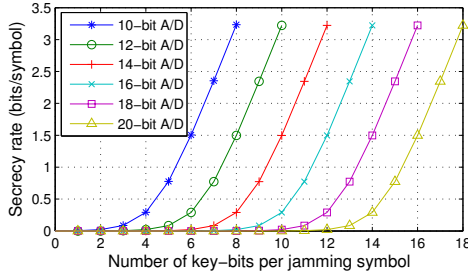
Fig. 5. Achievable secrecy rates versus the number of key bits for 10-bit A/D at Bob and various qualities of Eve's A/D. P = 1 , l = 2.5 , and the signal-to-noise ratio of both Eve's and Bob's channels is 30 dB.
