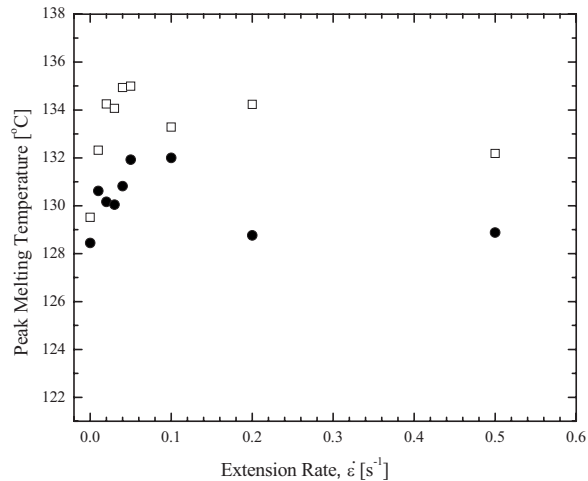
FIG. 9. Peak melting temperature as a function of extension rate for isotactic poly-1-butene samples at T_c=98^\circ\text{C} . Included are the solutions for DP0401M ( \square ) at a fixed strain of \varepsilon=5.0 and PB 0200 ( \bullet ) at a fixed strain of \varepsilon=4.0 .
