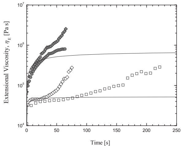
FIG. 3. FiSER measurements of the transient extensional viscosity as a function of time for different extension rates of poly-1-butene at T=98^{\circ}\text{C} . Included are the solutions of extension rates of \dot{\epsilon}=0.01\text{ s}^{-1} ( \square ), 0.02\text{ s}^{-1} ( \bullet ), and 0.03\text{ s}^{-1} ( \blacklozenge ). The open symbols correspond to DP0401M and filled symbols correspond to PB0200. The linear viscoelastic response is superimposed over the data.
