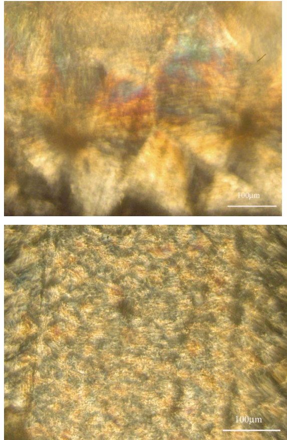
FIG. 6. Microscopy images taken through crossed polarizers of the DP0401M samples showing the size and alignment of crystals under (a) quiescent conditions ( \dot{\epsilon}=0.0 \text{ s}^{-1} ) and (b) following a stretch with an extension rate of \dot{\epsilon}=0.05 \text{ s}^{-1} and an accumulated strain of \epsilon=5 . The stretch direction is aligned vertically.
