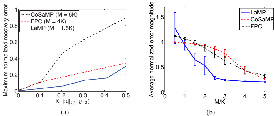
Figure 5: Performance of LaMP. (a) Maximum recovery error over 100 noise iterations as a function of the input noise variance. LaMP has the same robustness to noise as the FPC and CoSaMP algorithms. (b) Performance over background subtraction dataset of 100 images. LaMP achieves the best performance at M \approx 2.5K , while both FPC and CoSaMP require M > 5K to achieve the same performance.
