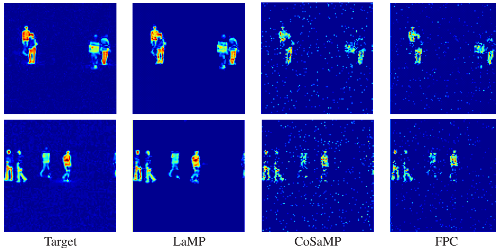
Figure 6: Example recoveries for background subtraction images, using M = 3K for each image. processing applications, signals are acquired merely for the purpose of making an inference such as a detection or classification decision.
