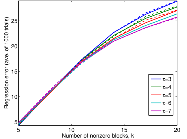
Figure 3: Performances of the group lasso for designs with varying spectral norms and extremal coherence values (cf. Table 2) in regression of block-sparse vectors as a function of the number of nonzero regression blocks k ; \tau denotes the value of the spectral norm multiplier used. Solid lines correspond to X 's with minimum coherence, while dashed lines correspond to X 's with maximum coherence.
