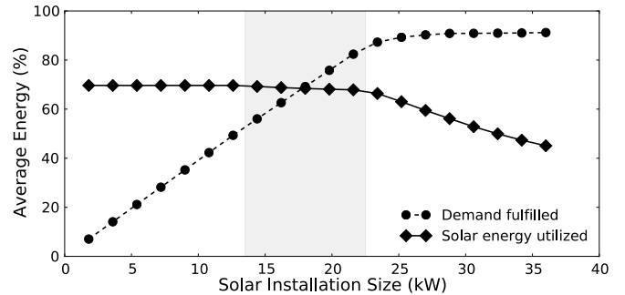
Fig. 9. Variable solar installation size with average solar utilization and demand fulfillment using the synthetically constructed dataset.
