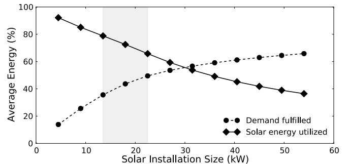
Fig. 10. Energy demand fulfilled and solar utilized using the real-world dataset for the entire year. The highlighted region shows the typical PV systems size that can be installed in a parking lot for 5 cars.
