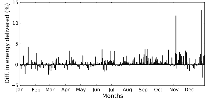
Fig. 8. Difference in overall energy estimated by the offline and the energy delivered by the online approach to the cars using real-world dataset for the entire year
