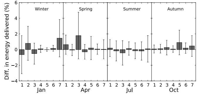
Fig. 7. Difference in overall energy estimated by the offline and the energy delivered by the online approach to the cars with poisson arrival rate of 2 cars per hour
