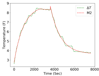
Figure 6: An example of an M2 (screen use) model and the empirical T_B - T_A M2 curve.
