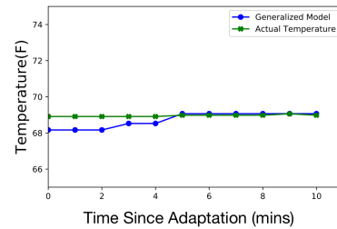
Figure 12: Ambient temperature prediction for a warming curve beyond the training phase after adjusting the parameters using domain adaptation.
