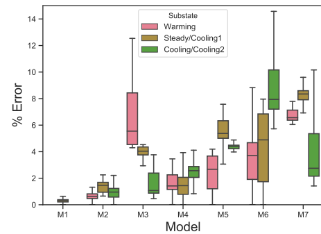
Figure 9: Errors (in %) of temperature predictions across model states and sub-states.
