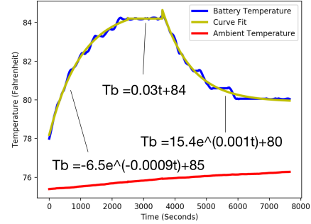
Figure 2: Exponential warming, linear steady state, and exponential cooling fit to battery temperature as it rises and falls in our M2 (screen use) experiment.
