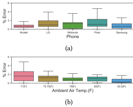
Figure 10: Errors (in %) of M2 (screen use) temperature predictions for a range of (a) devices and (b) ambient temperatures.
