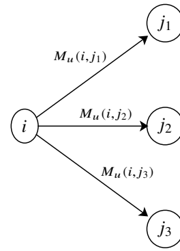
Fig. 5: If the total number of visits to State i is M_i(u) = m_i(u) , then the number of visits from state i to states j_k ( M_u(i, j_k) ) follow a multinomial distribution with probabilities p_u(i, j_k) .
