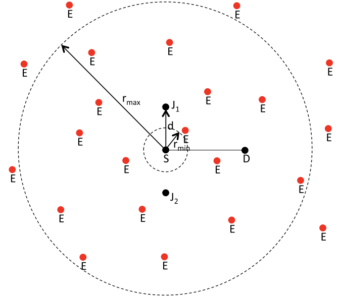
Fig. 2. One-hop communication between source S and destination D in the presence of eavesdroppers ( E_s ). In SMER, two jammers J_1 and J_2 help to make the link secure.
