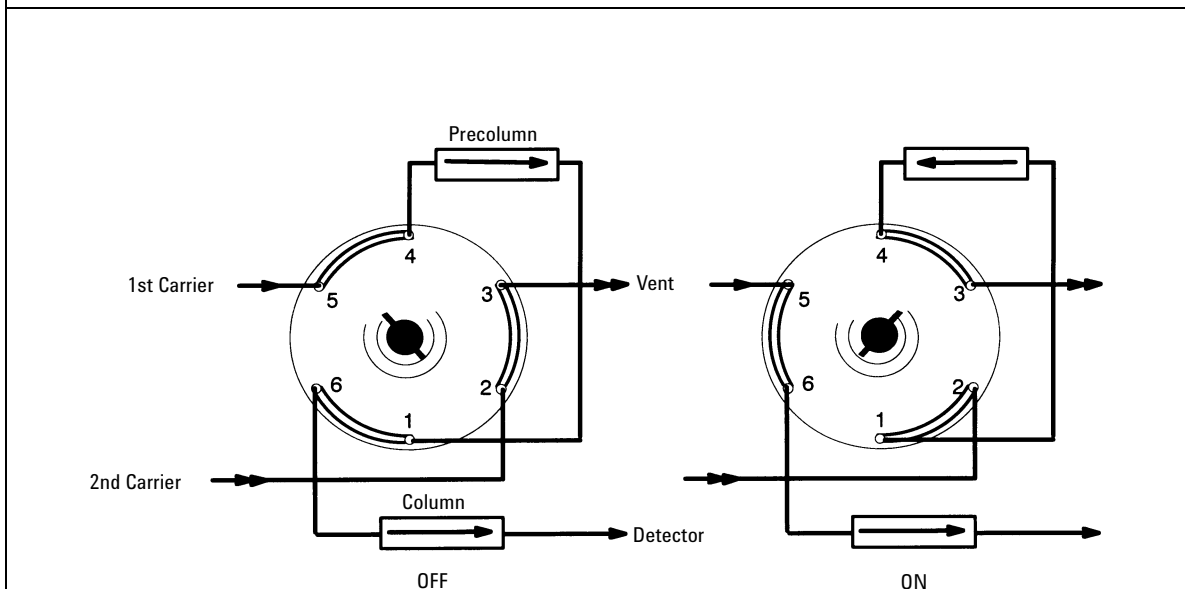
Backflush a Precolumn to Vent, Option 705 or 735
