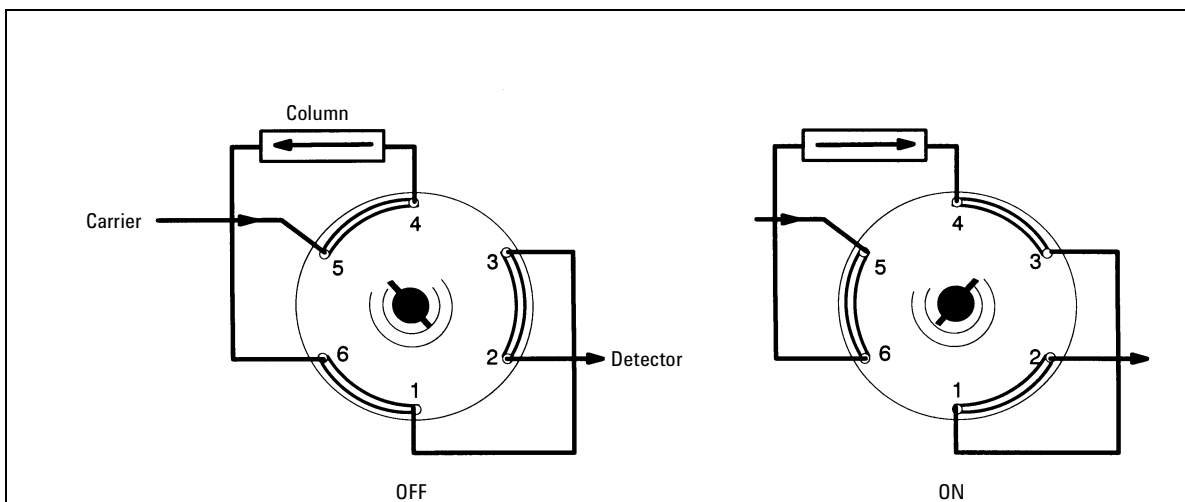
Backflush to Detector, Option 704 or 734
