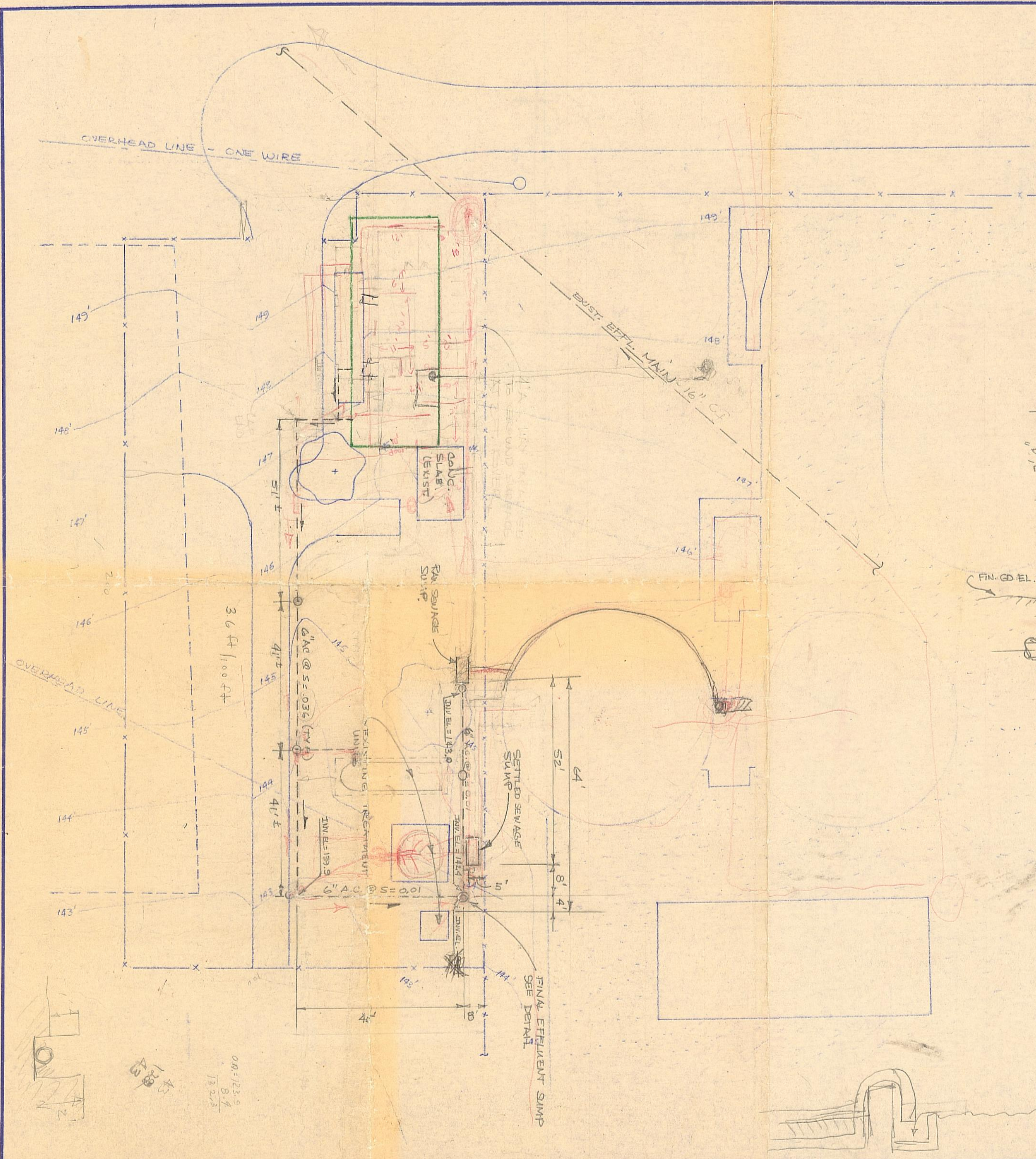
SETTLED SEWAGE SUMP DETAIL
