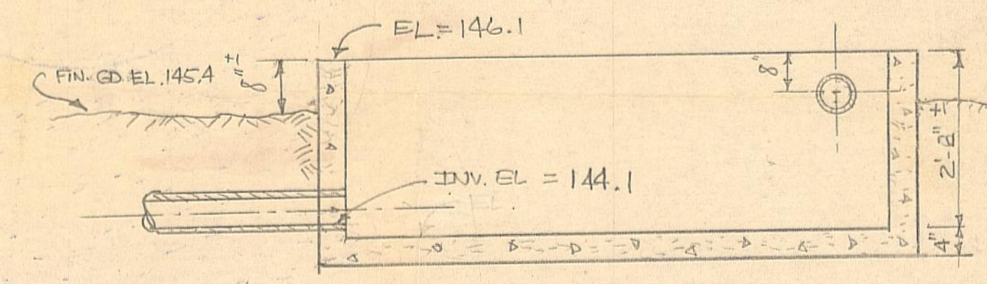
SETTLED SEWAGE SUMP DETAIL
