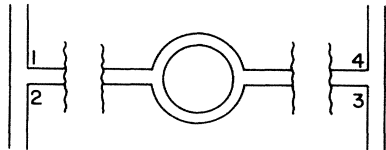
FIG. 2. Loop connected to leads longer than an inelastic scattering length. Phase randomization is introduced by the two reservoirs to the left and right of the loop. The Aharonov-Bohm oscillations of this conductor are symmetric.
