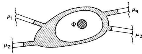
FIG. 1. Disordered normal conductor with four terminals connected via perfect leads (unshaded) to four reservoirs at chemical potentials \mu_1 , \mu_2 , \mu_3 , and \mu_4 . An Aharonov-Bohm flux \Phi is applied through the hole of the sample.
