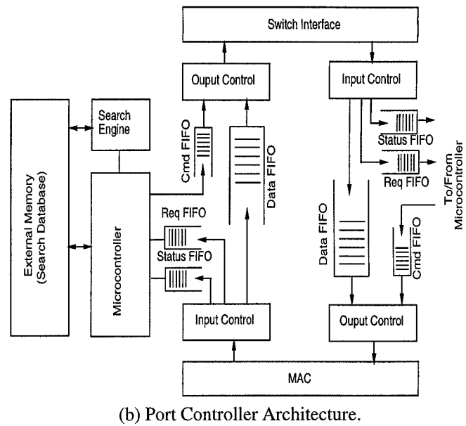
Fig. 1. Switch & Port Controller Architectures.
