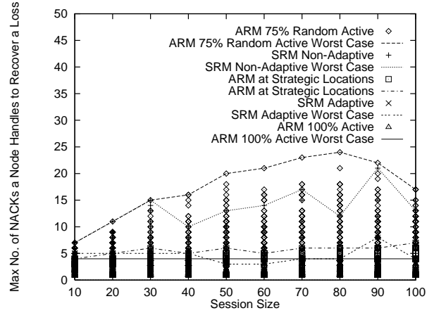
Fig. 3. NACK implosion control (loss near source, 1000 nodes, degree 4). ARM caches repairs, but not fresh data packets.
