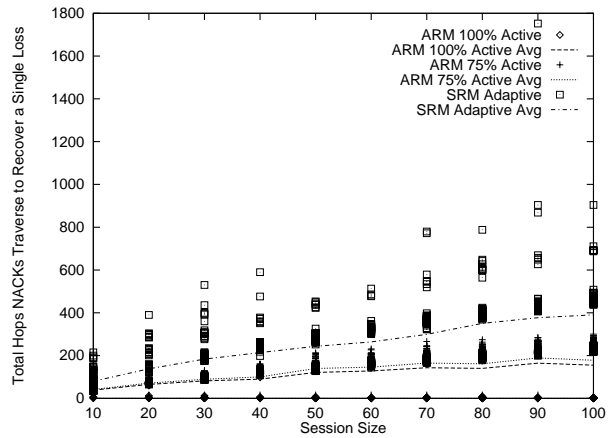
Fig. 4. NACK bandwidth consumption (loss near source, 1000 nodes, degree 4). ARM caches repairs, but not fresh data packets. SRM uses adaptive algorithm.
