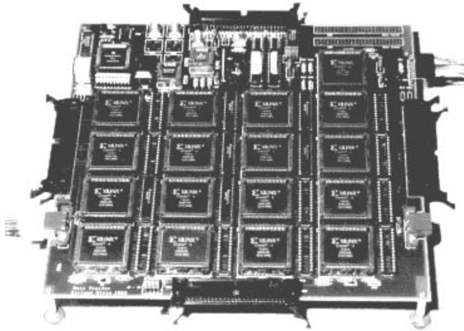
Figure 21: Virtual Wires Emulation Board
