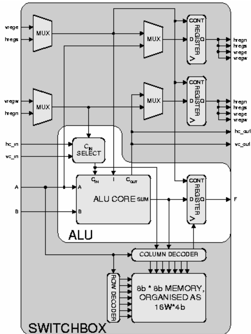
Figure 4 Logical structure of an ALU and switchbox
