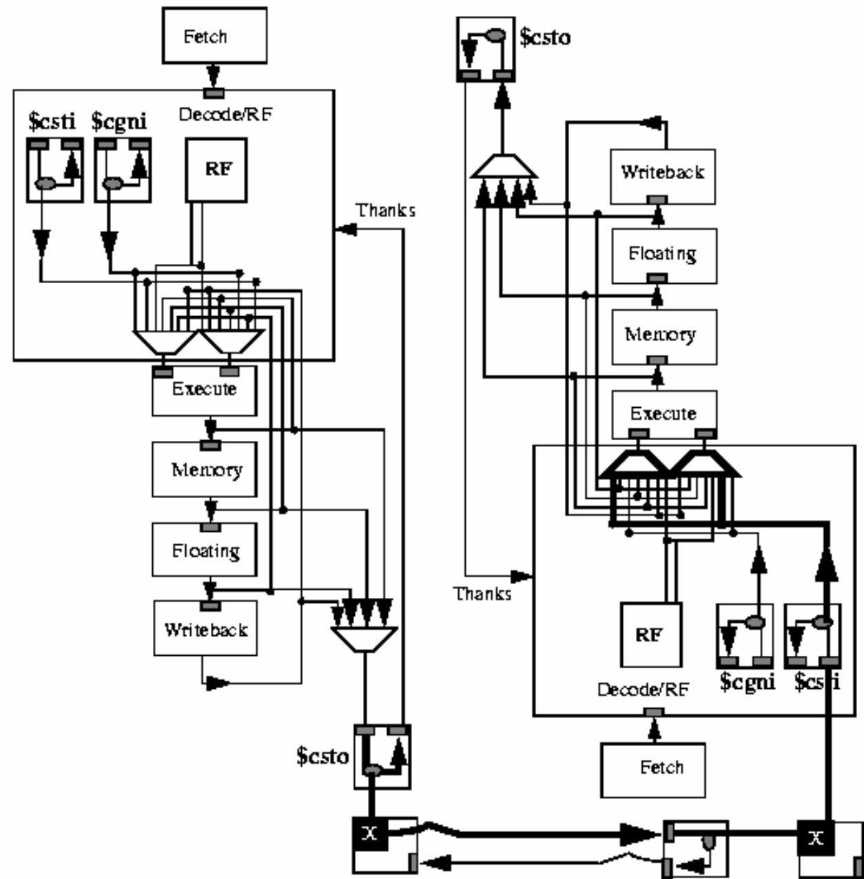
The Processor-Switch-Switch-Processor path
