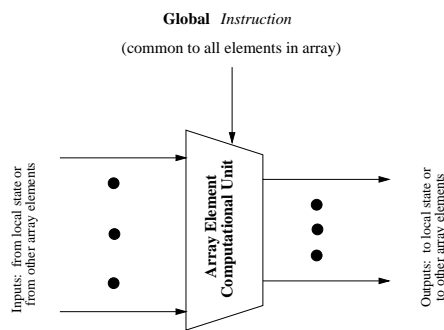
Figure 4: Computational Unit for SIMD AE
