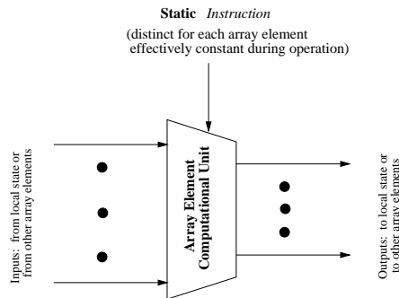
Figure 3: Computational Unit for FPGA AE
