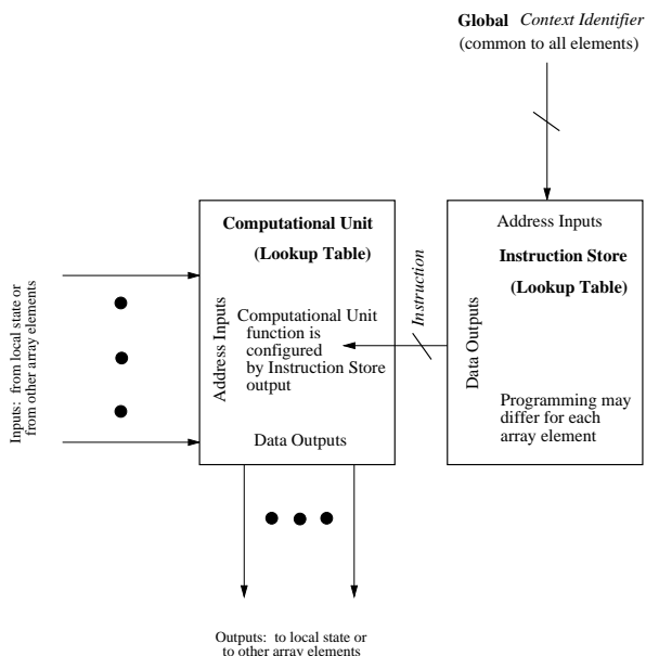
Figure 6: Configurable Instruction-Store View of DPGA AE
