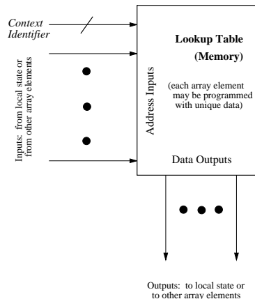
Figure 5: Lookup Table Model for DPGA
