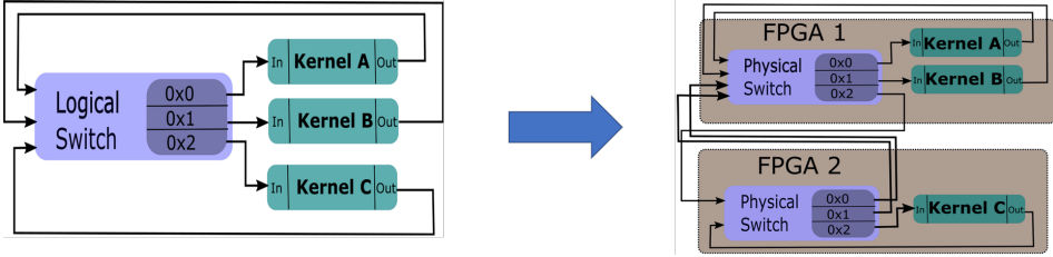
Fig. 4. The logical view of the cluster from the user's perspective is transformed with the Galapagos Middleware into a multi-FPGA implementation [212].
