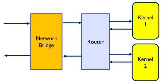
Fig. 5. Bridges and routers generated by the Middleware placed on each FPGA.
