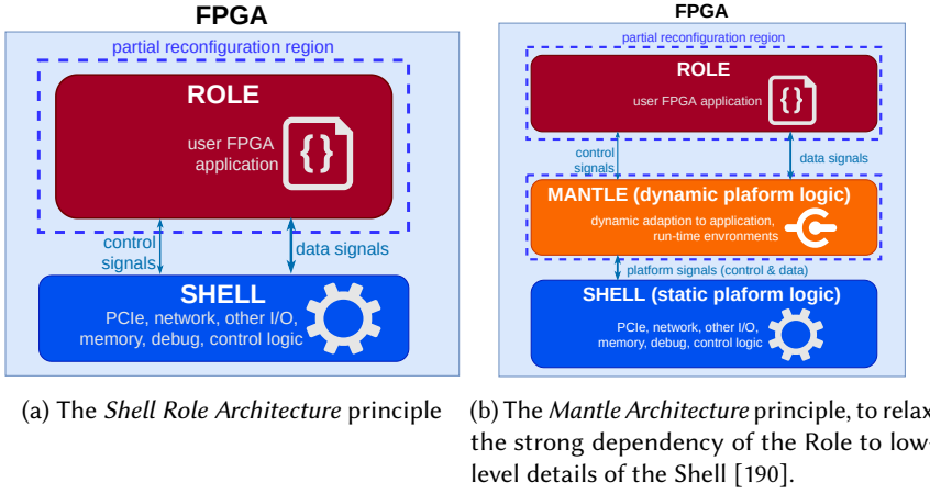
Fig. 3. Shell Role and Mantle Architecture Principle
