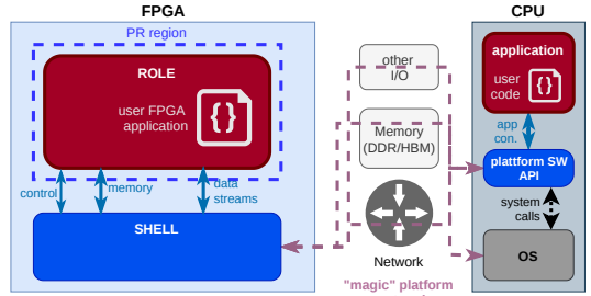
Fig. 6. Shell Role Architecture share many common concepts.
