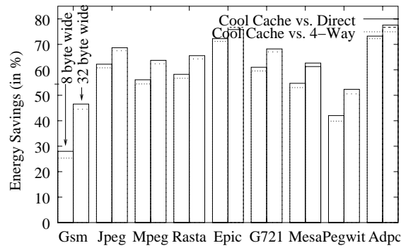
(a) 8-Byte and 32-Byte wide SRAM Cool-Cache 16-register CPU
