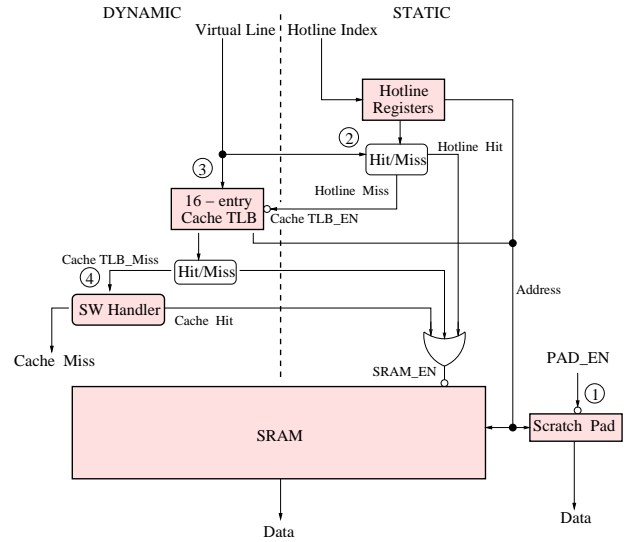
Figure 1. The Cool-Cache Architecture
