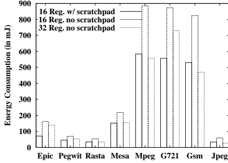
Figure 5. 16-register architecture with scratchpad can be more energy efficient than 32-register architecture without scratchpad.
