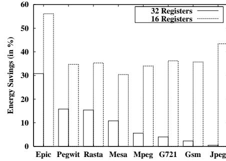
Figure 4. Scratchpad Energy Savings.
