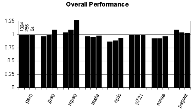
Figure 11. Cool-Cache performance
