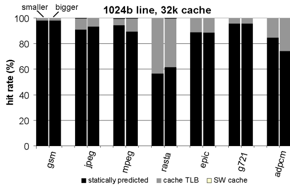
Figure 9. Hit rate sensitivity to benchmark input
