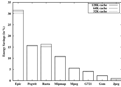
(b) Energy savings
