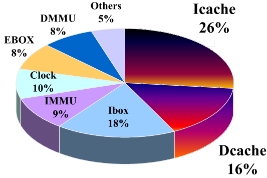
(a) StrongARM (Source: IEEE JSCC, Nov.96)
