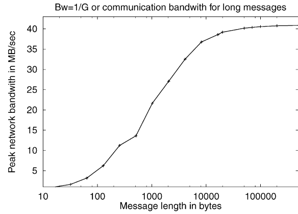
Fig. 5. Network bandwidth, 1/G , for different message sizes. For sufficiently large messages (over about 10 Kbytes), the network bandwidth can be approximately as constant.
