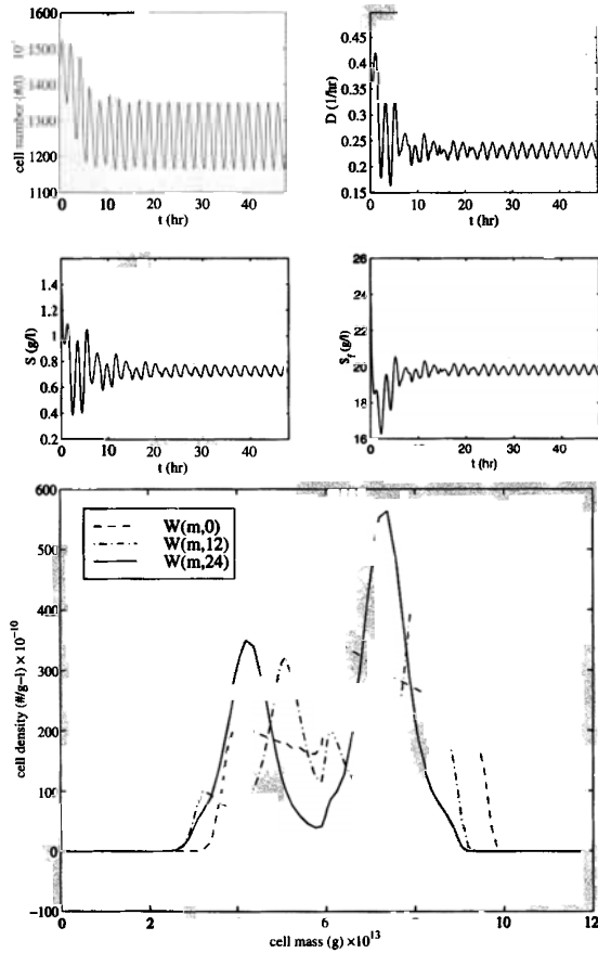
Figure 6: Oscillation stabilization with LMPC control.
