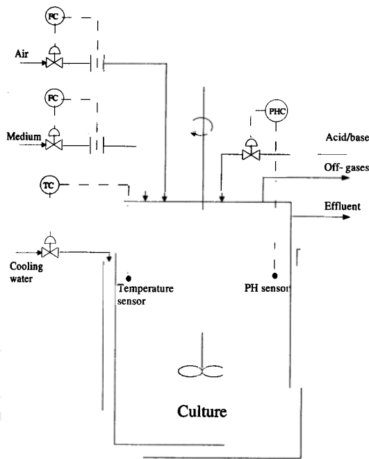
Figure 1: Continuous bioreactor.
