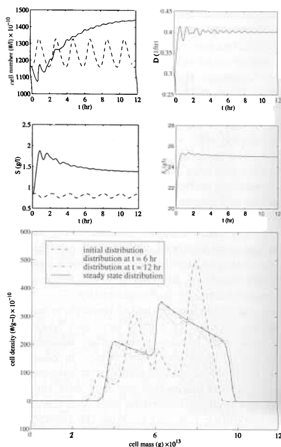
Figure 5: Oscillation attenuation with LMPC control.
