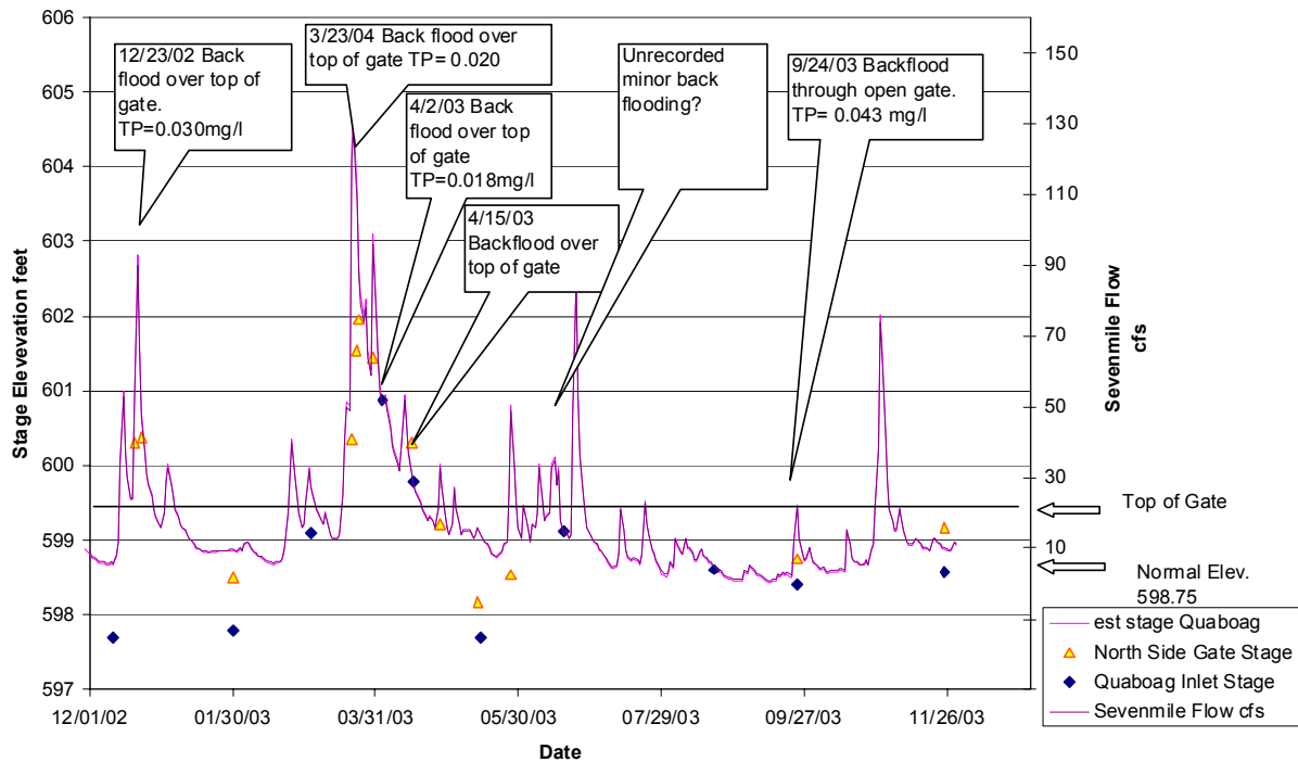
Figure 13. Water Stage at Quaboag Pond and at Quacumquisit gate. Water stage level shown as points. The line represents the instantaneous flow rate at the USGS gage on the Sevenmile River at Cooney Road.
