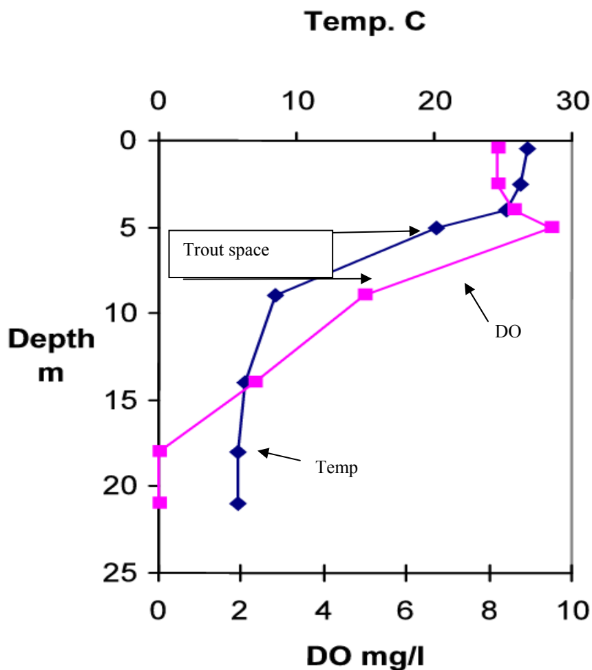
Figure 10. Quacumquasit Pond DO and Temperature 8/20/03.
