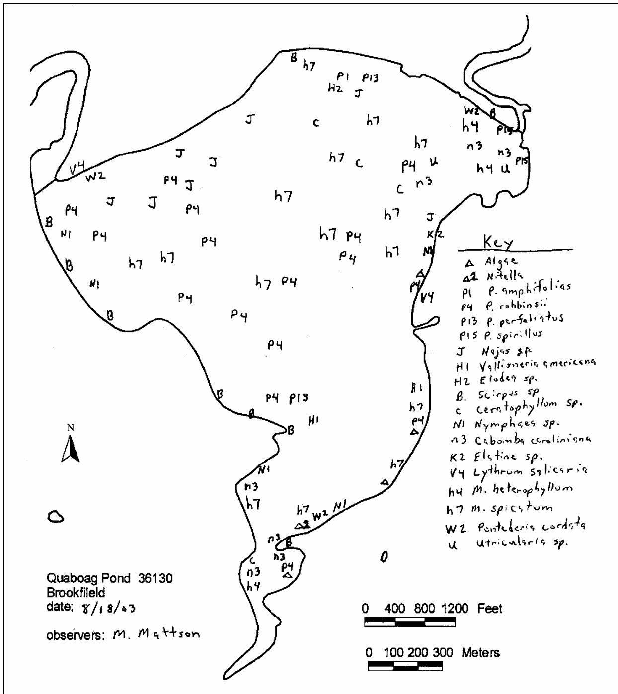
Figure 8. Quaboag Pond Macrophyte Species distribution (2003).
