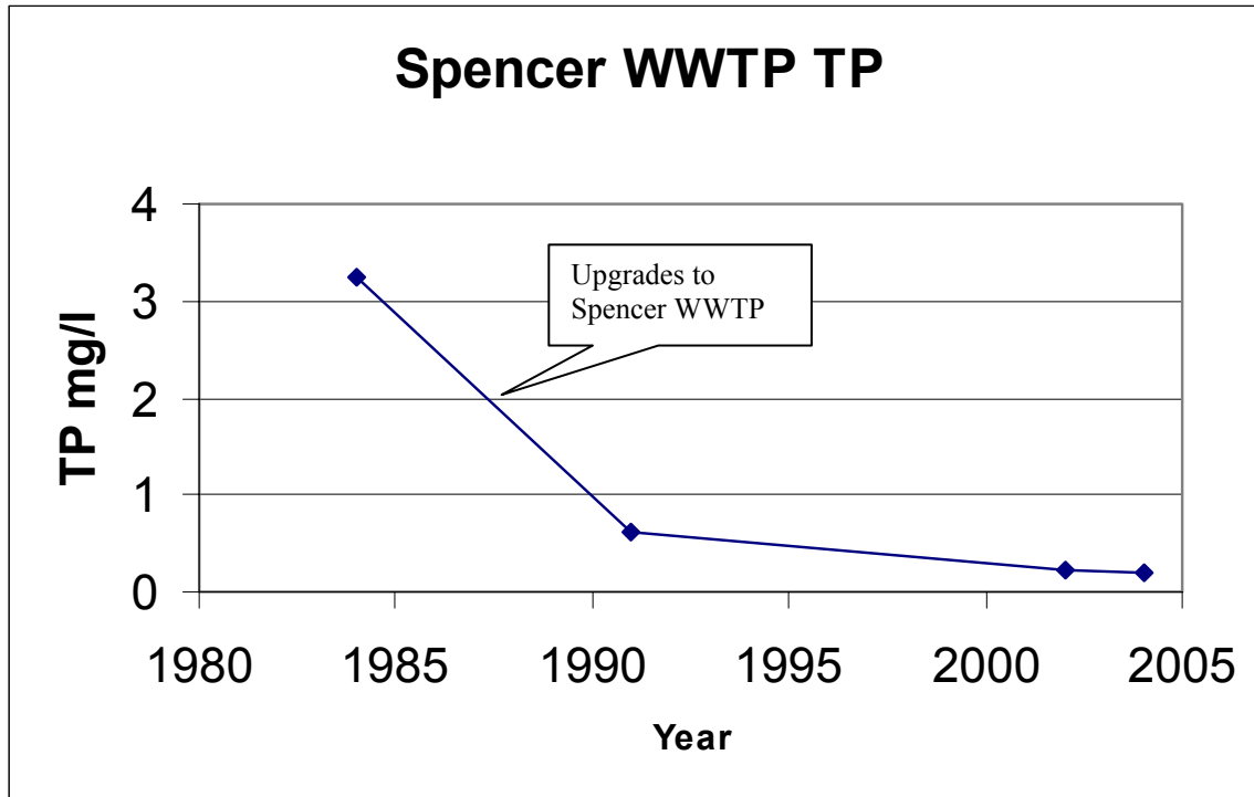
Figure 3. Trend in Total Phosphorus in effluent of Spencer WWTP.
