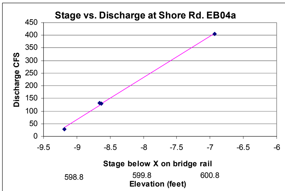
Figure D 1. Stage vs. Discharge at Site EB04a Shore Road.
