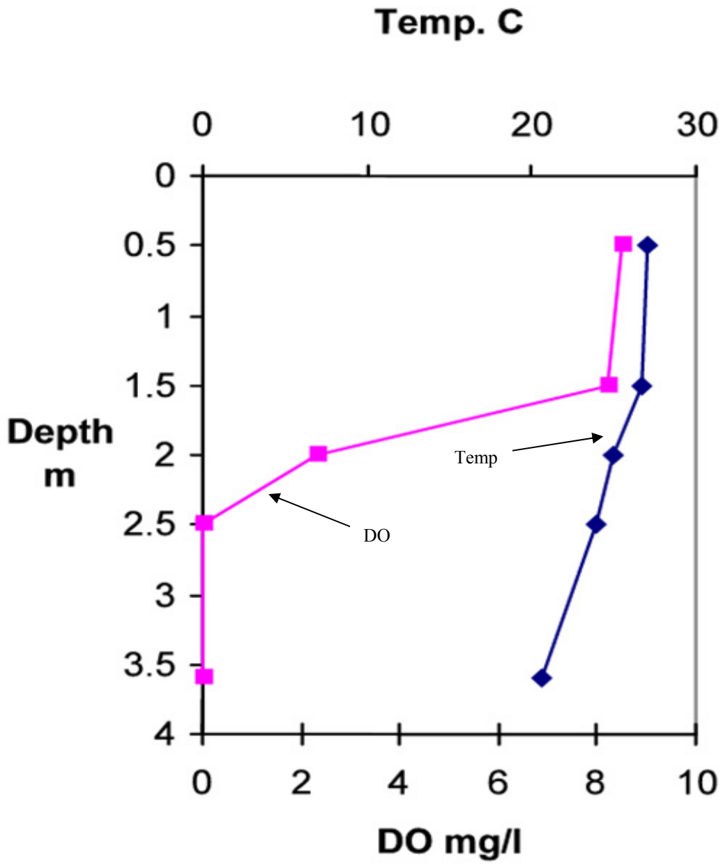
Figure 4. Quaboag Pond DO and Temperature 8/20/03.
