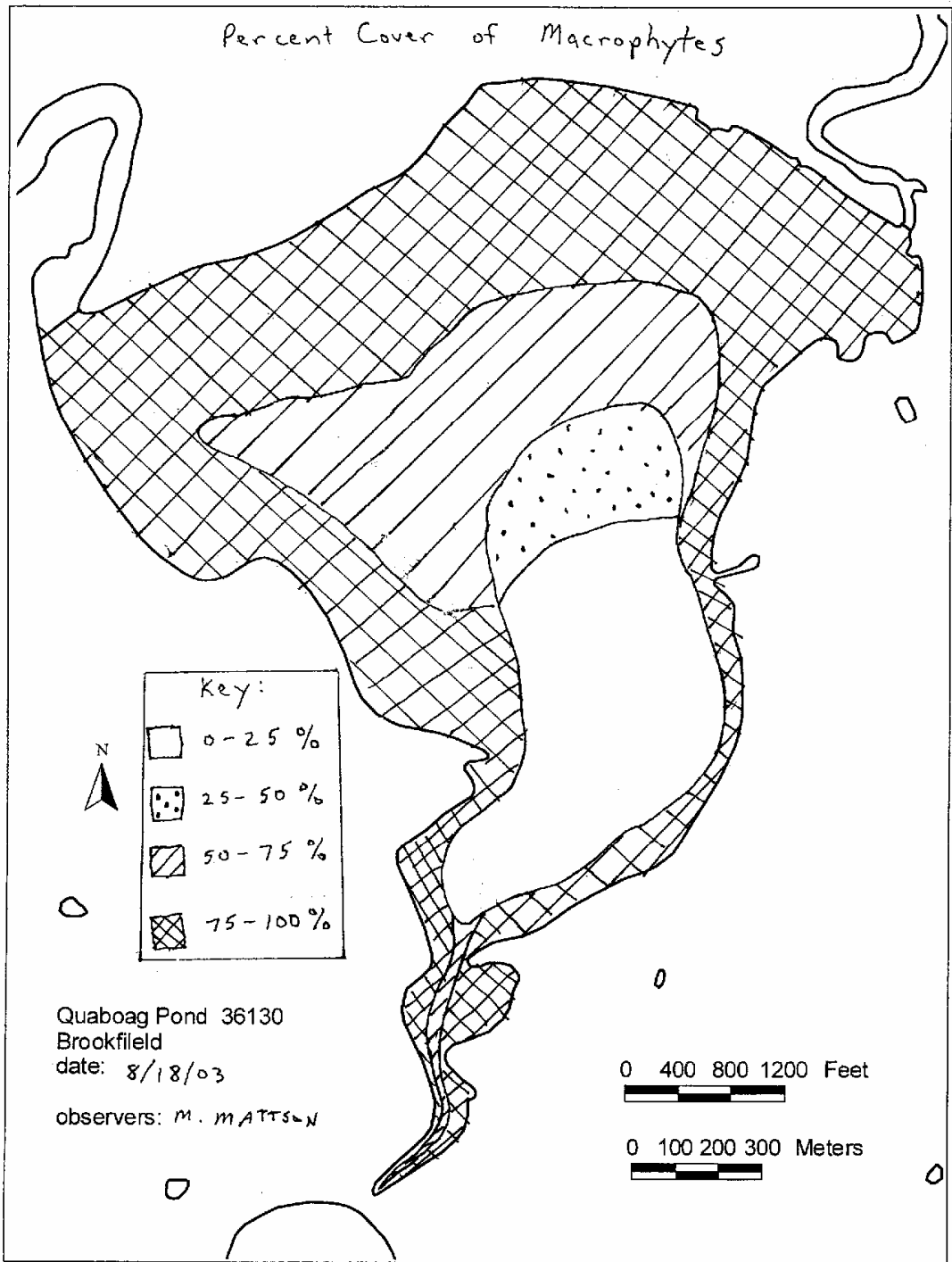
Figure 6. Quaboag Pond Macrophyte distribution (2003).
