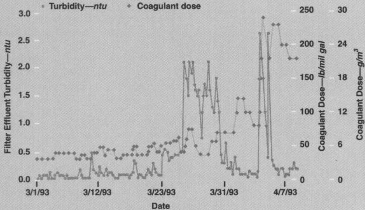
FIGURE 2 Combined filter effluent turbidity and coagulant dose at the Howard Avenue plant—spring 1993
