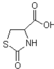
2-Oxothiazolidine-4-carboxylic acid
