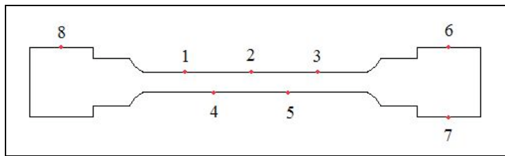
Figure 1. Hardness test locations.
