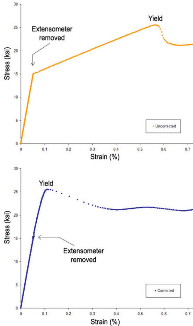
Figure 4. Uncorrected and corrected stress strain diagrams.
