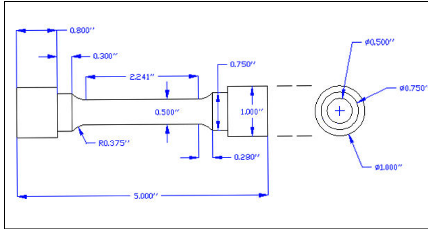
Figure 2. Tension coupon dimensions.
